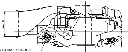
OPTIONAL DRY BREAK FITTINGS CP6300-21 TIGHTENING TORQUE 13Nm DRY BREAK TO BE USED IN CONJUNCTION WITH CP6300-7 BLEED SYSTEM FITTING. FOR FURTHER DRY BREAK INFORMATION & SPARES REFER TO CP6300-13CD INSTALLATION DRAWING.
