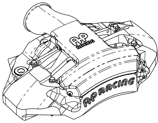
OPTIONAL DRY BREAK FITTINGS CP6300-21 TIGHTENING TORQUE 13Nm DRY BREAK TO BE USED IN CONJUNCTION WITH CP6300-7 BLEED SYSTEM FITTING. FOR FURTHER DRY BREAK INFORMATION & SPARES REFER TO CP6300-13CD INSTALLATION DRAWING.
