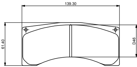
CP6821D46 FAMILY IRON PAD AREA - 61.70M 2 THICKNESS - 1.6CM VOLUME - 61.7CM 3
