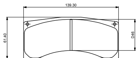
CP6820D46 FAMILY IRON PAD AREA - 61.7CM 2 THICKNESS - 1.6CM VOLUME - 67.9CM 3
