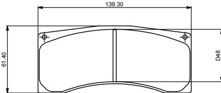
CP6820D48 FAMILY IRON PAD AREA - 63.2CM 2 THICKNESS - 1.6CM VOLUME - 69.5CM 3
