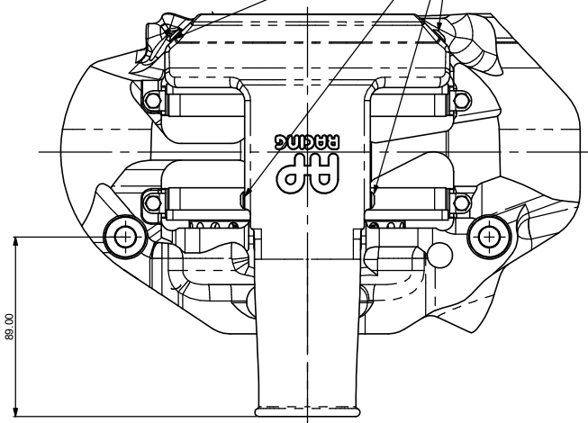
5x M4x0.70 BUTTON HEAD SCREWS (INCLUDED IN DUCT KIT)
